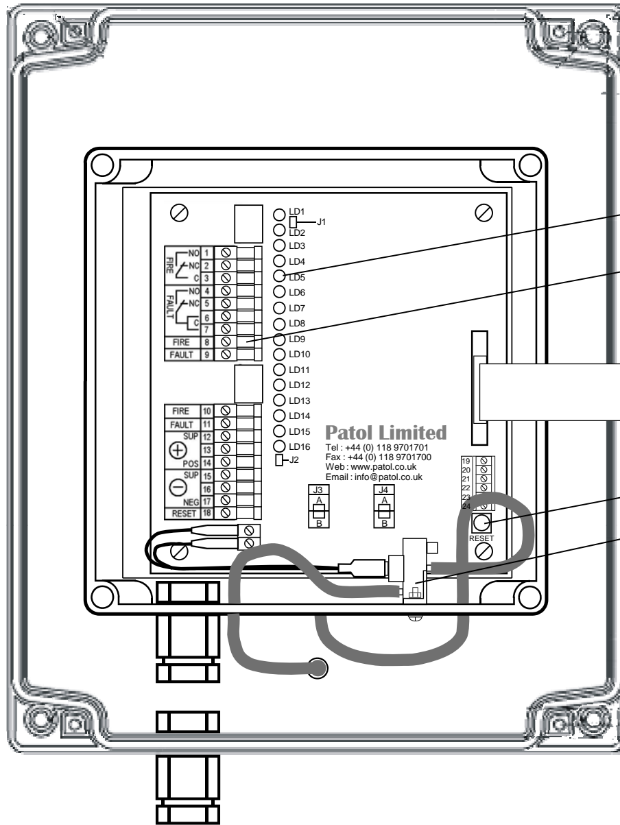
INTERNAL VIEW - OUTER LID & FASCIA REMOVED
