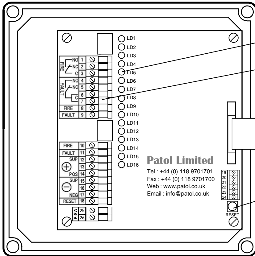
INTERNAL VIEW - FASCIA REMOVED
