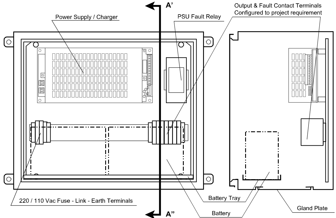
INTERNAL VIEW ( Door Removed)
